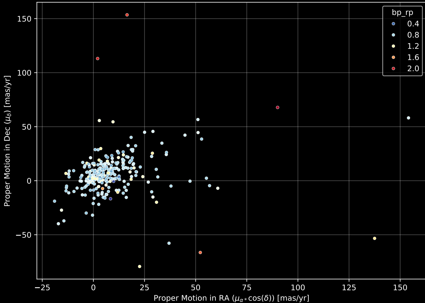
GALAH DR4 Field: [129] Proper Motion Diagram (n= 289)
