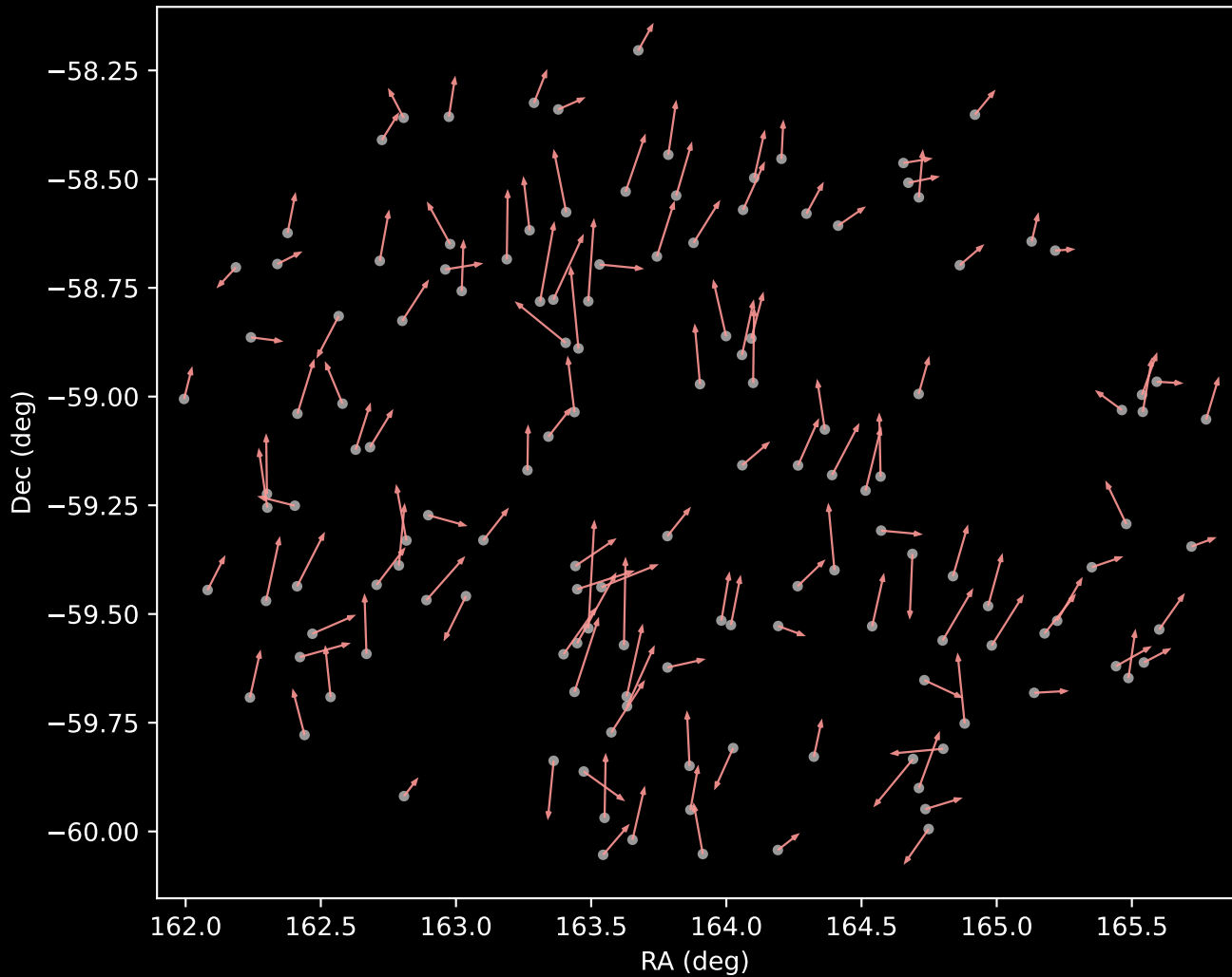
GALAH DR4 Cluster 7 Proper Motion Vectors (n=140)
