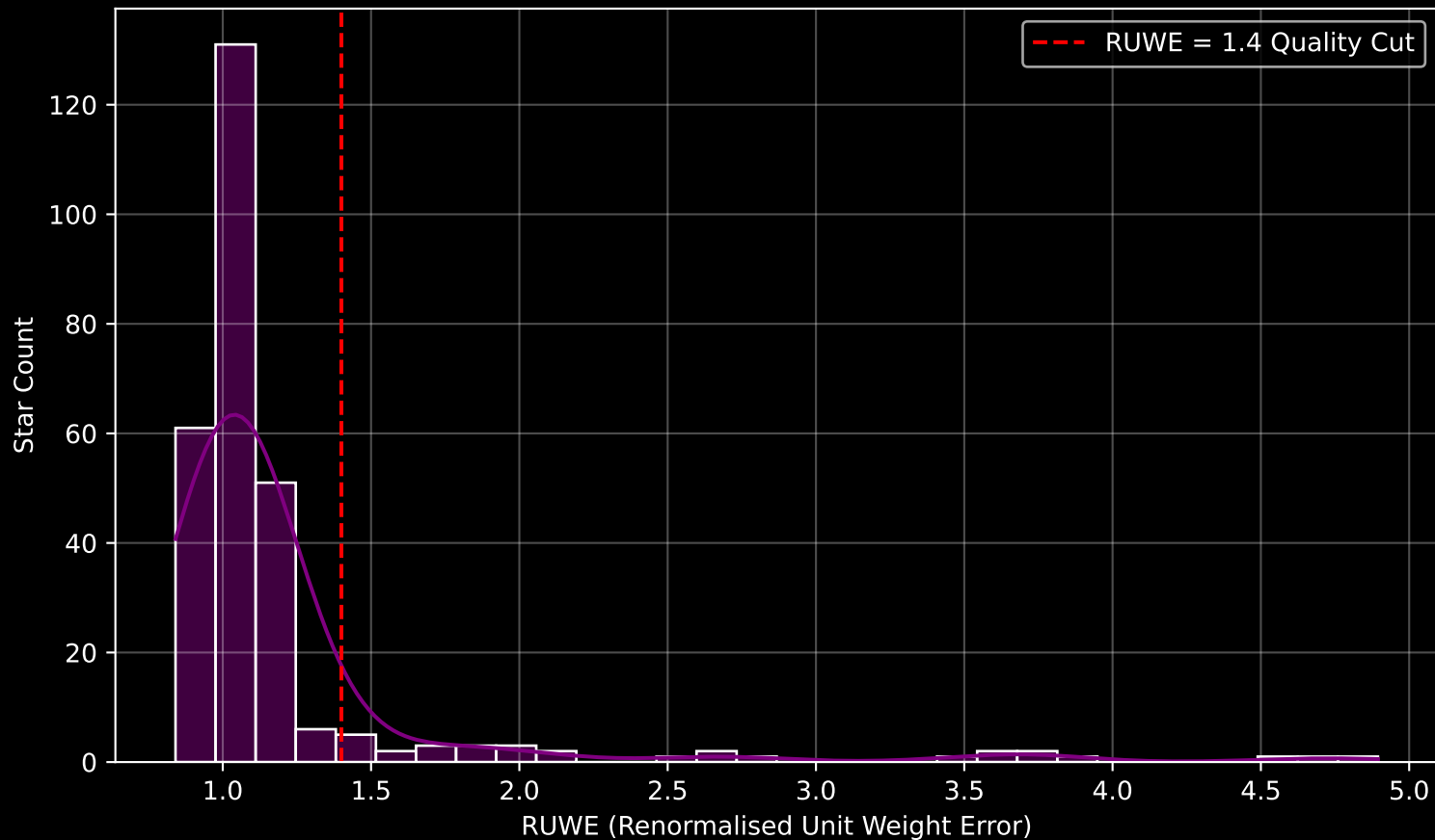
GALAH DR4 Field [129] RUWE Distribution (n= 280)
