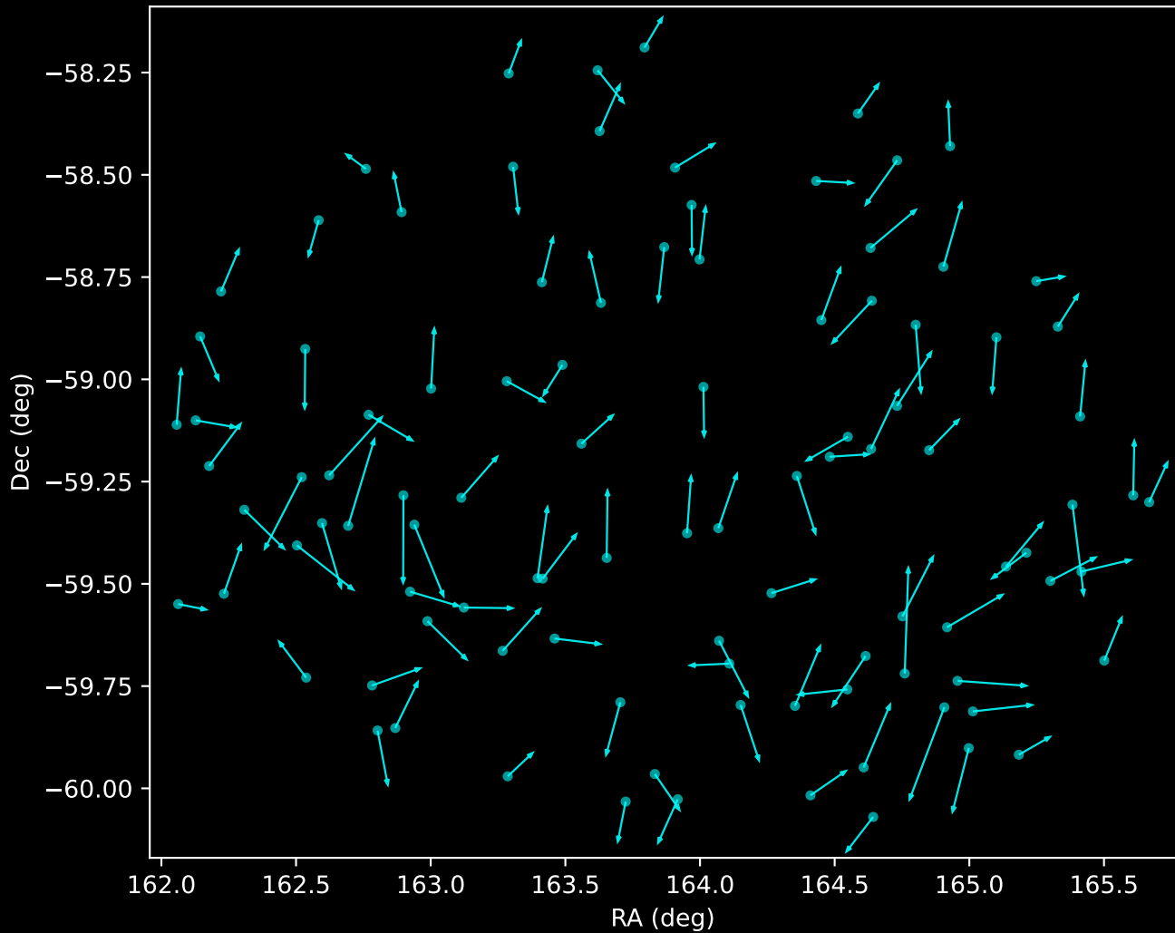
GALAH DR4 Noise Stream Proper Motion Vectors (n=101)
