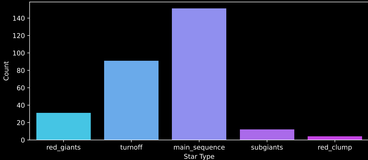
GALAH DR4 Field: [129] Count plot of Star Type
